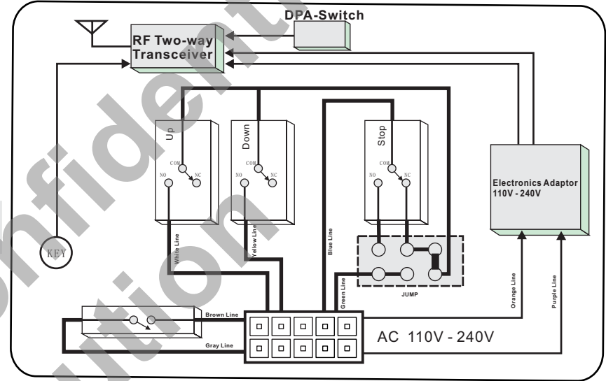
Garage Door Remote Controls Block Diagram
