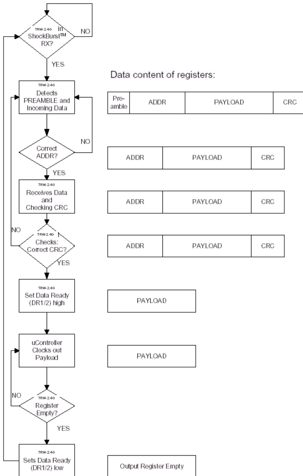
Figure 6 Flow Chart ShockBurst™ Receive of TRW-24G.
