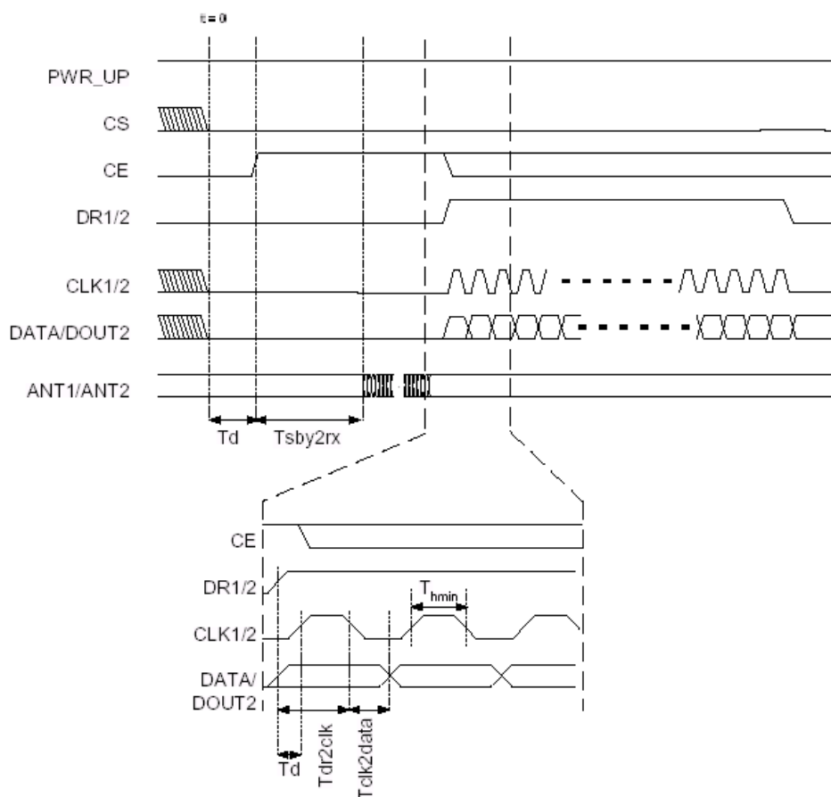
Figure13 Timing of ShockBurst™ in RX
